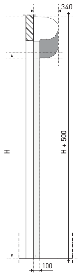
[ Dwarsdoorsnede ]
