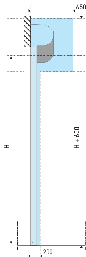
[ Dwarsdoorsnede ]
