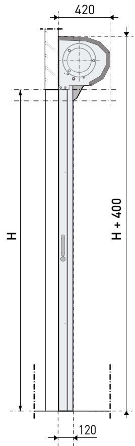
[ Dwarsdoorsnede ]
